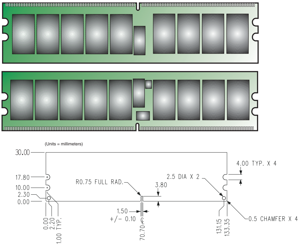
Figure 1: KVR400D2D4R3/4G 240-Pin DIMM
